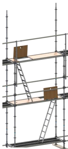
Figure 8.18 : Garde-corps MDS monté
