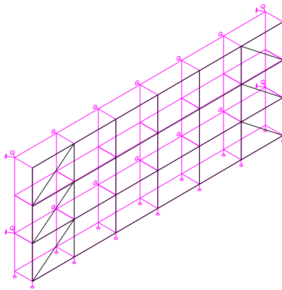
Figure 6.7 : Diagonale verticale
